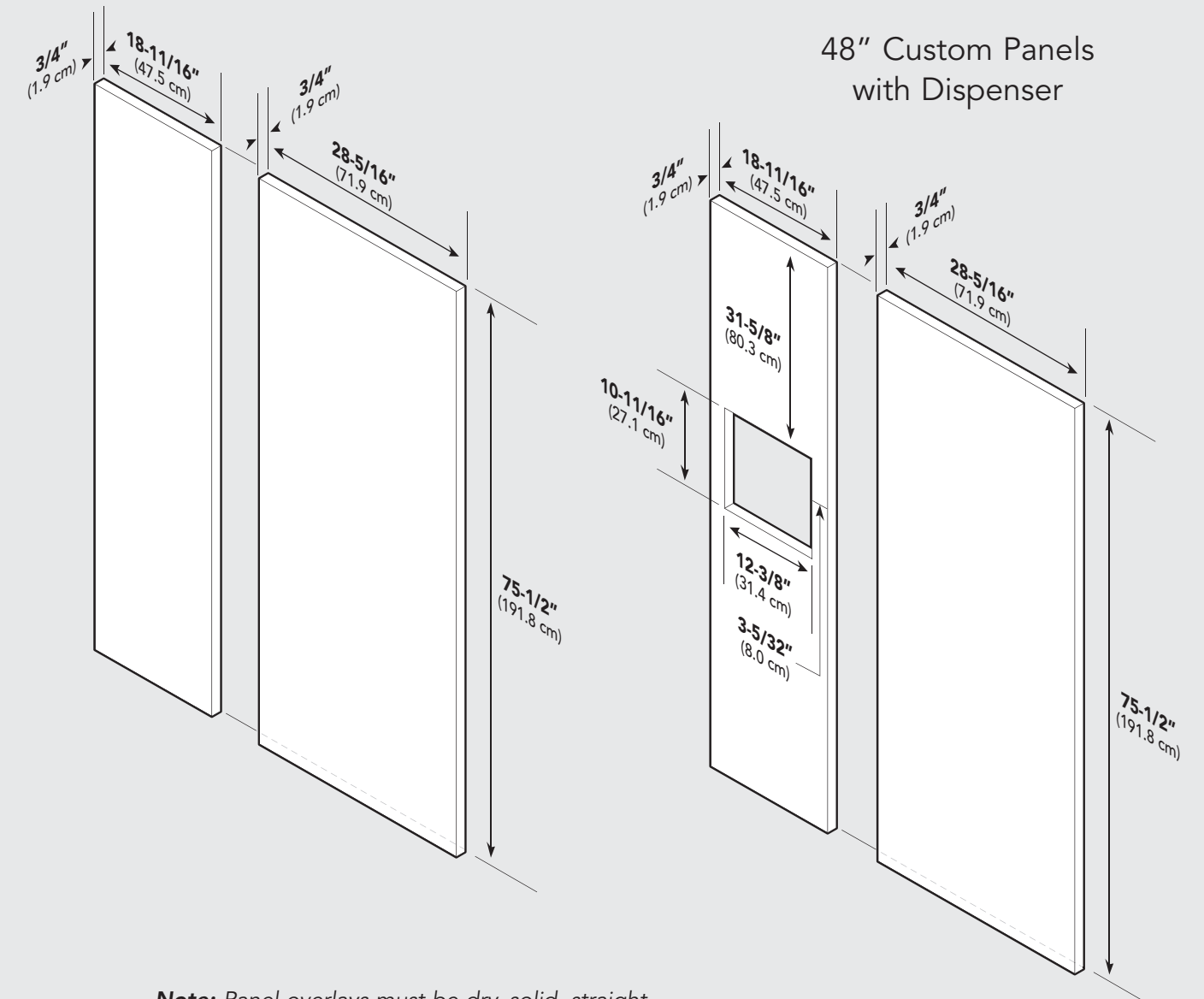
48" Custom Panels
