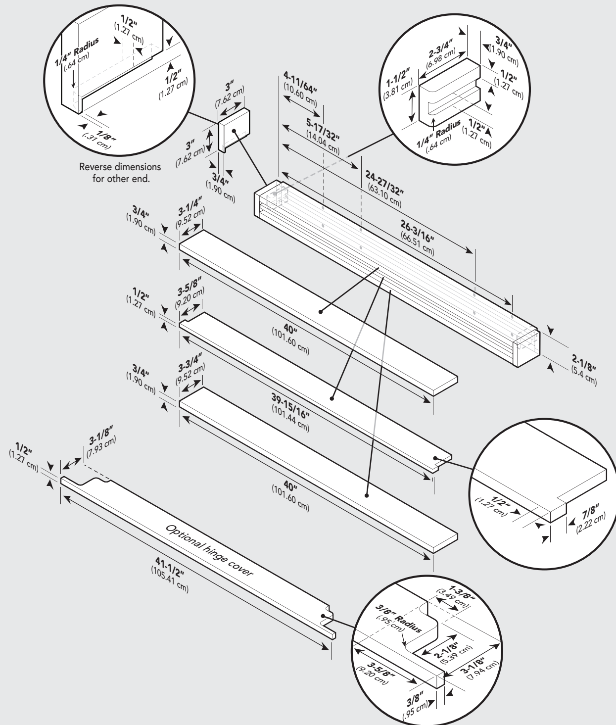
42" Custom Grille
