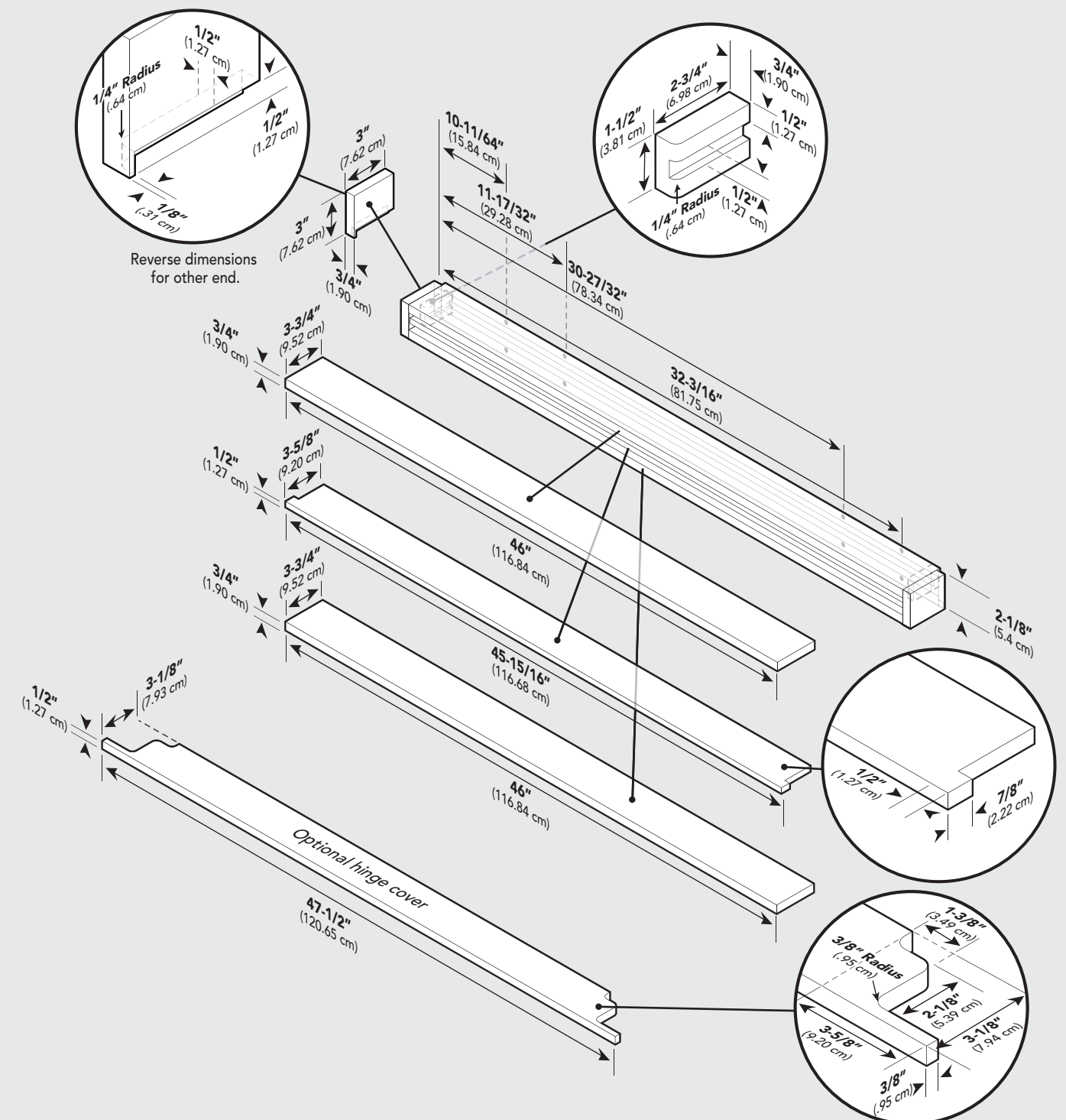
48" Custom Grille
