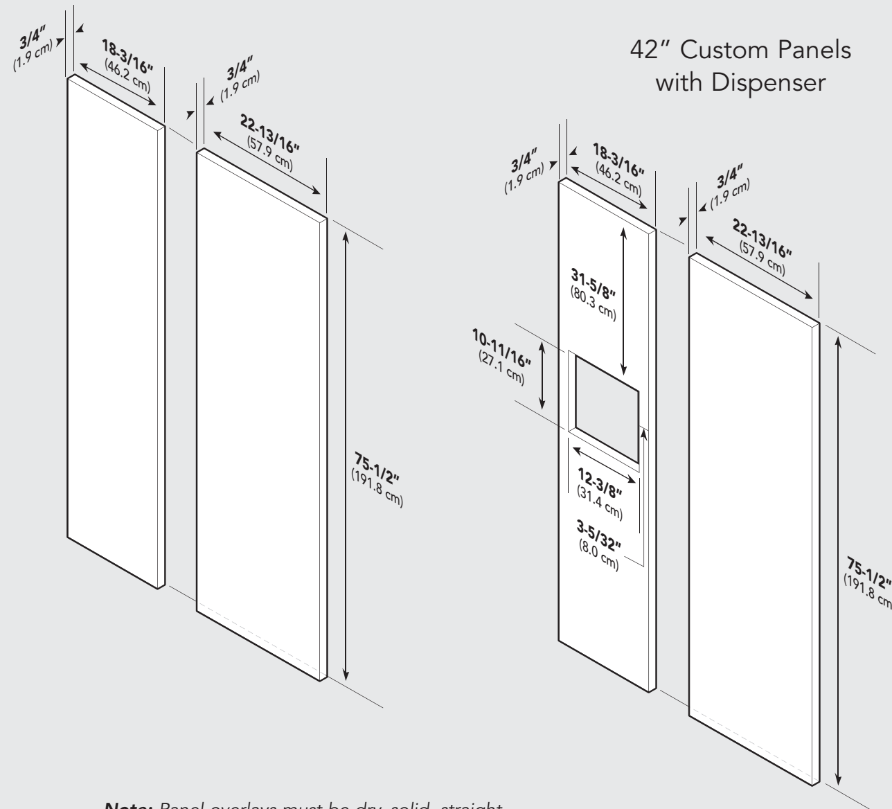
42" Custom Panels
