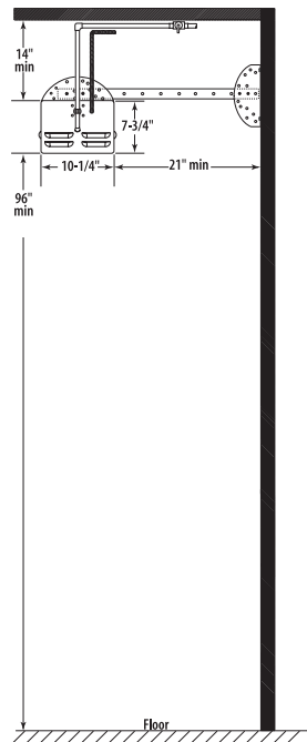
0° installation to combustible surface (side view)
