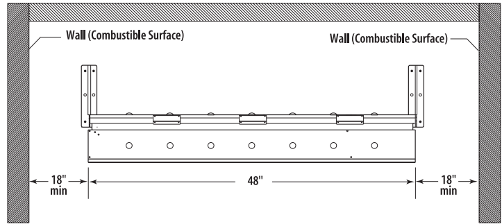
0° installation to combustible surface (side view)
