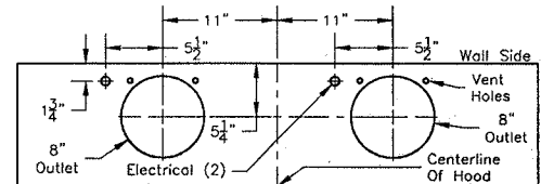
1200 CFM Double B200 Dual Blowers (Top View)
