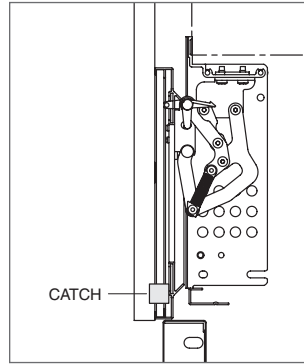
Catch (side view).
