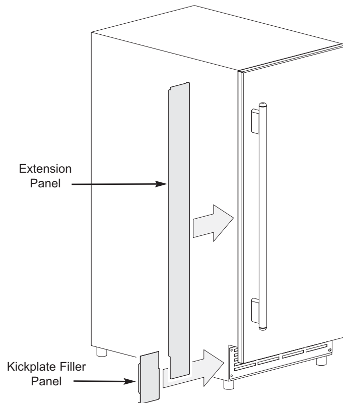
Figure 1. UC15I Filler Panel Installation
