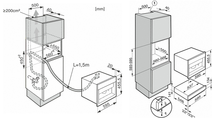
CVA5065, CVA6405, CVA6805, plumbed in water supply (installation drawings)
