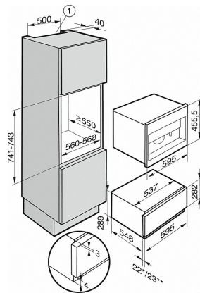
ESW 6129, ESW 6229 (Installation drawing)
